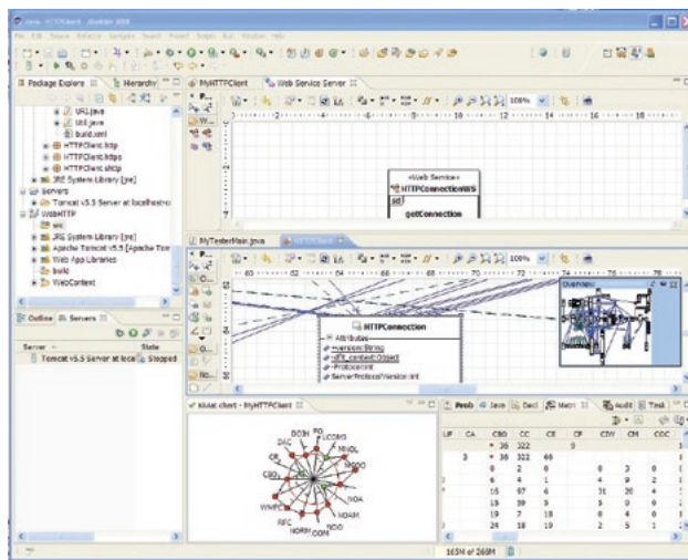
Exposing a web service in a Web services designer along with Kiviatt graph showing code metrics
